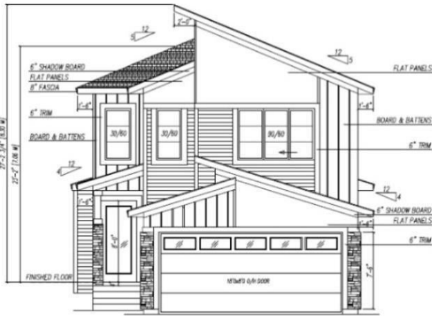
FRONT ELEVATION
